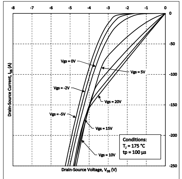
Figure 12. Body Diode Characteristics at T_J = 175^\circ\text{C}
