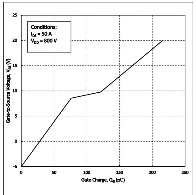
Figure 14. Gate Charge Characteristics
