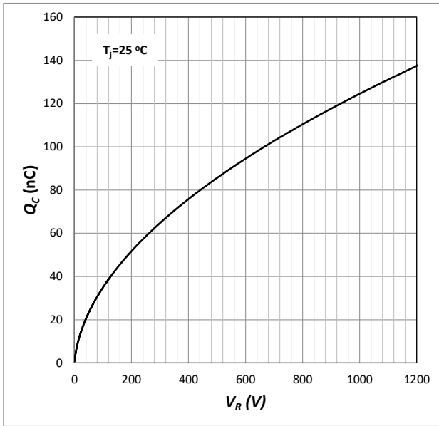
Fig. 7 Capacitive Charge
