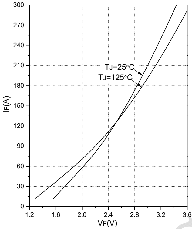
Fig.13 Forward Characteristics of Diode (Diode, Reverse)
