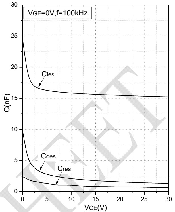
Fig.10 Capacitance Characteristics
