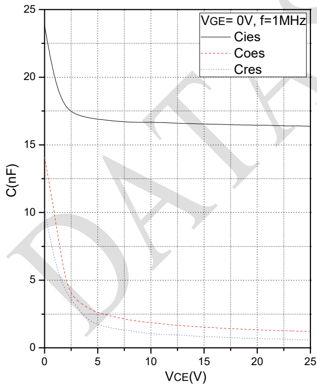
Fig.11 Capacitance Characteristics
