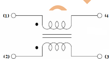
Equivalent Circuit
