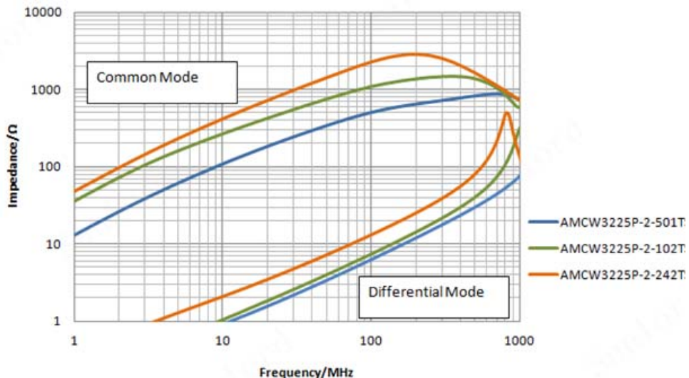
Impedance vs. Frequency
