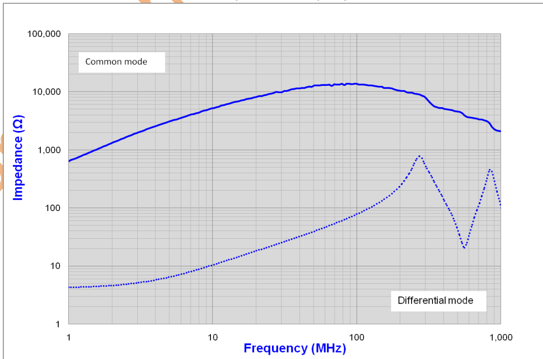
Impedance vs. Frequency
