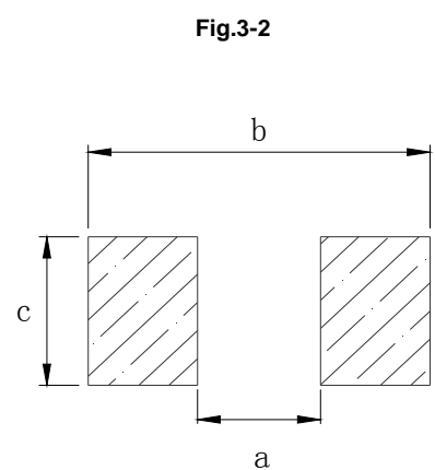
Recommend Land Pattern
