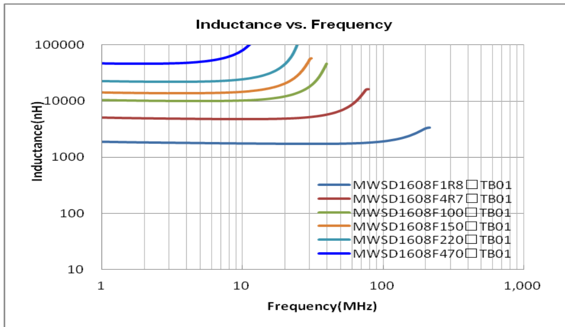
Inductance vs. Frequency Characteristics
