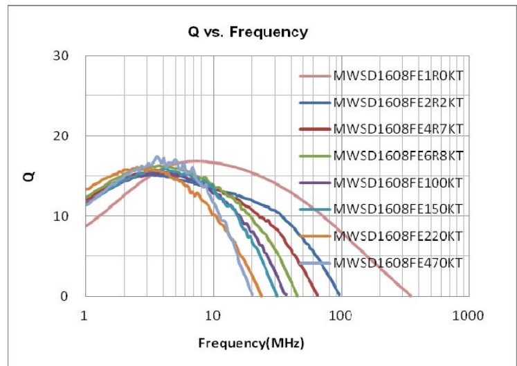
Q vs. Frequency Characteristics
