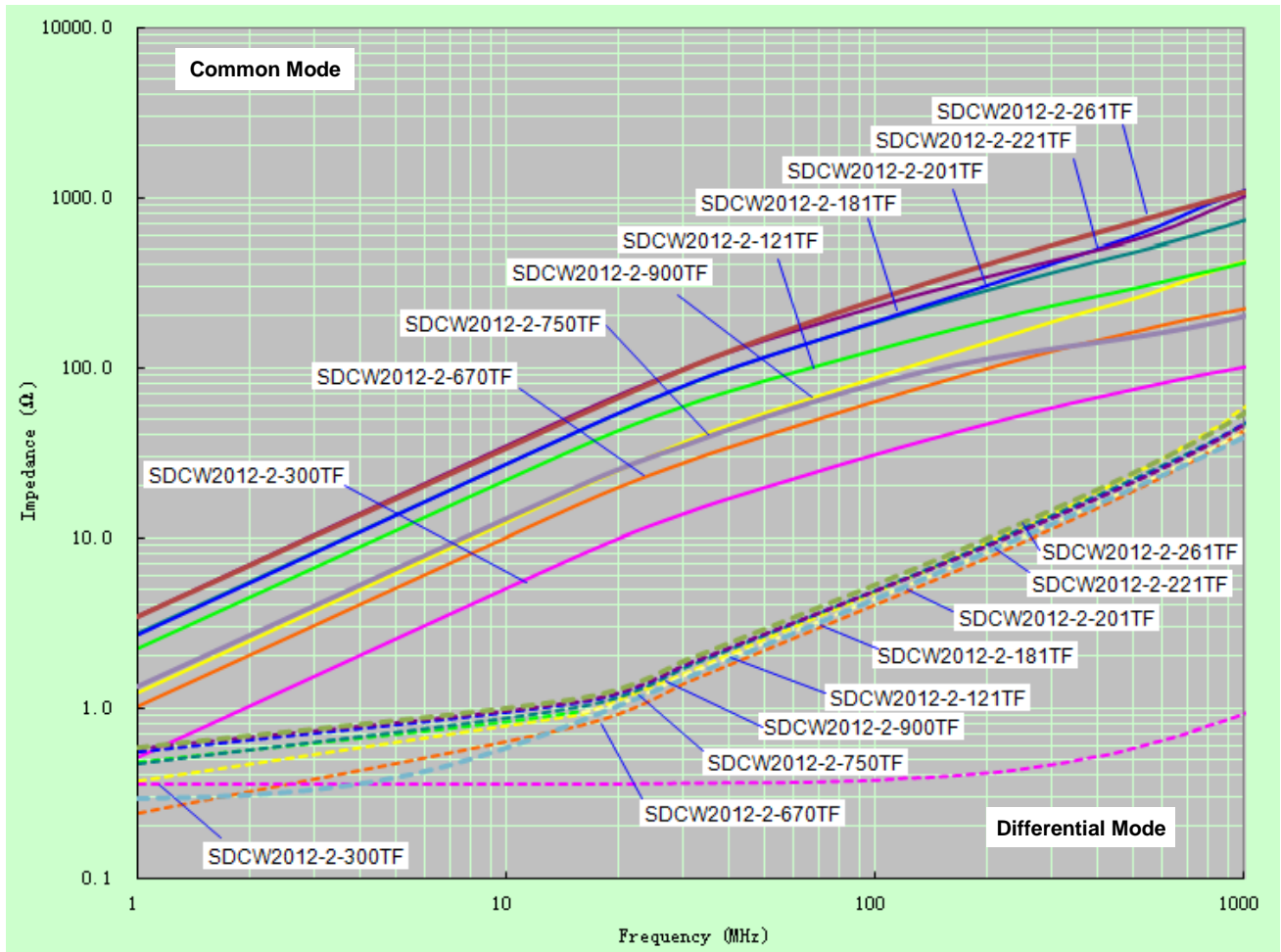
Impedance vs. Frequency (300~261)
