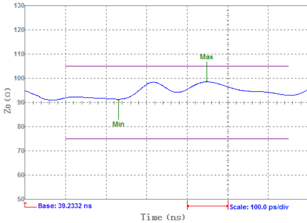
Characteristic Impedance
