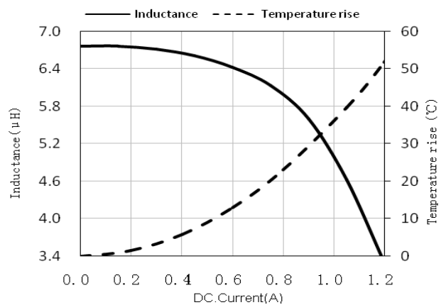
SPH252012H6R8MT
