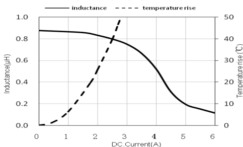
Typical Electrical Characteristics: SWPA4012SR82NT
