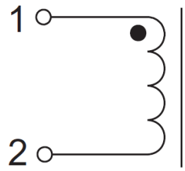
Fig.6-2 Schematic
