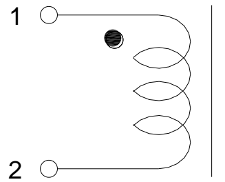
Fig.6-2 Schematic
