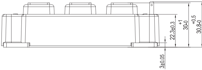
View A scale 3:1
