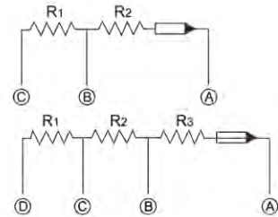
Circuit (电路图)
