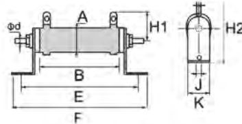
(QL Type 50W~600W)
