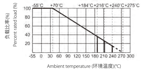
Derating Curve (降功率曲线)
